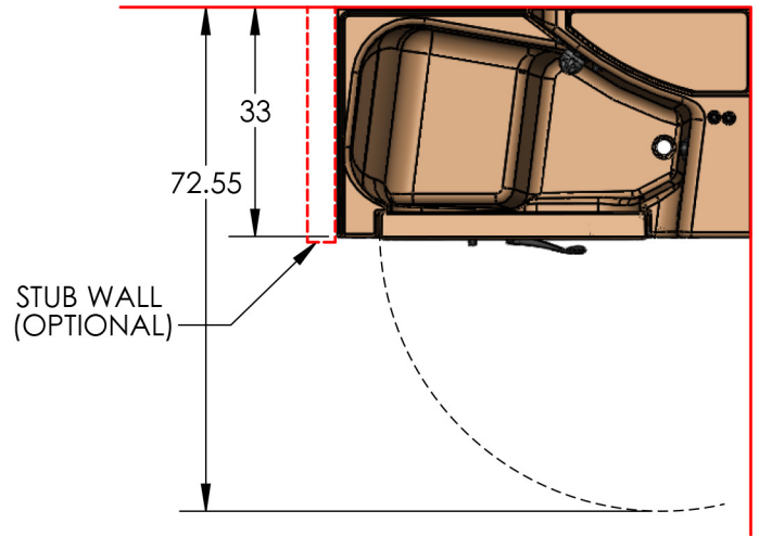
ALCOVE OR CORNER INSTALLATION
