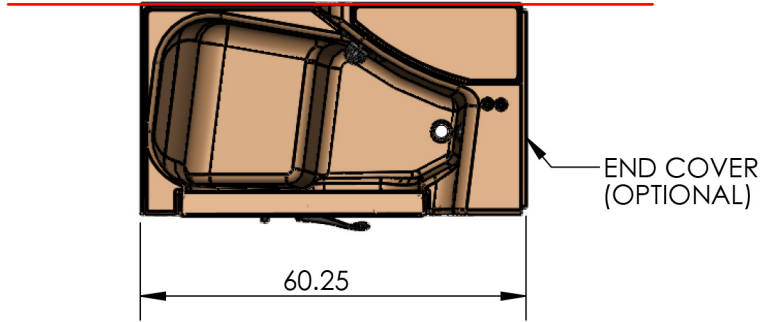
SIDE WALL INSTALLATION
